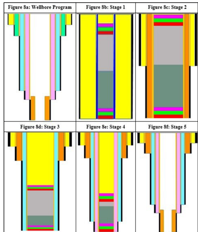
Figure 8. General wellbore diagram of each stage. Source: CEMPRI Software.
