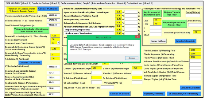
Figure 5. Calculation section on volumetry, additives, lead and tail volume, and others. Source: CEMPRI software.
