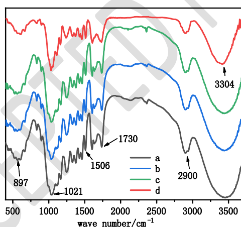
Figure 1: Infra-red spectrogram of untreated and pretreated bamboo shavings. (a) Untreated; (b) alkali treatment; (c) hydro-thermal treatment; (d) carbonizing treatment.
