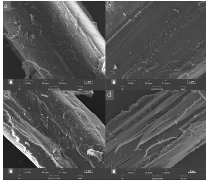
Figure 3: Scanning electron microscope graph of untreated and pretreated bamboo shavings. (a) Untreated (b) Carbonizing treatment (c) Hydro-thermal treatment (d) Alkali treatment.
