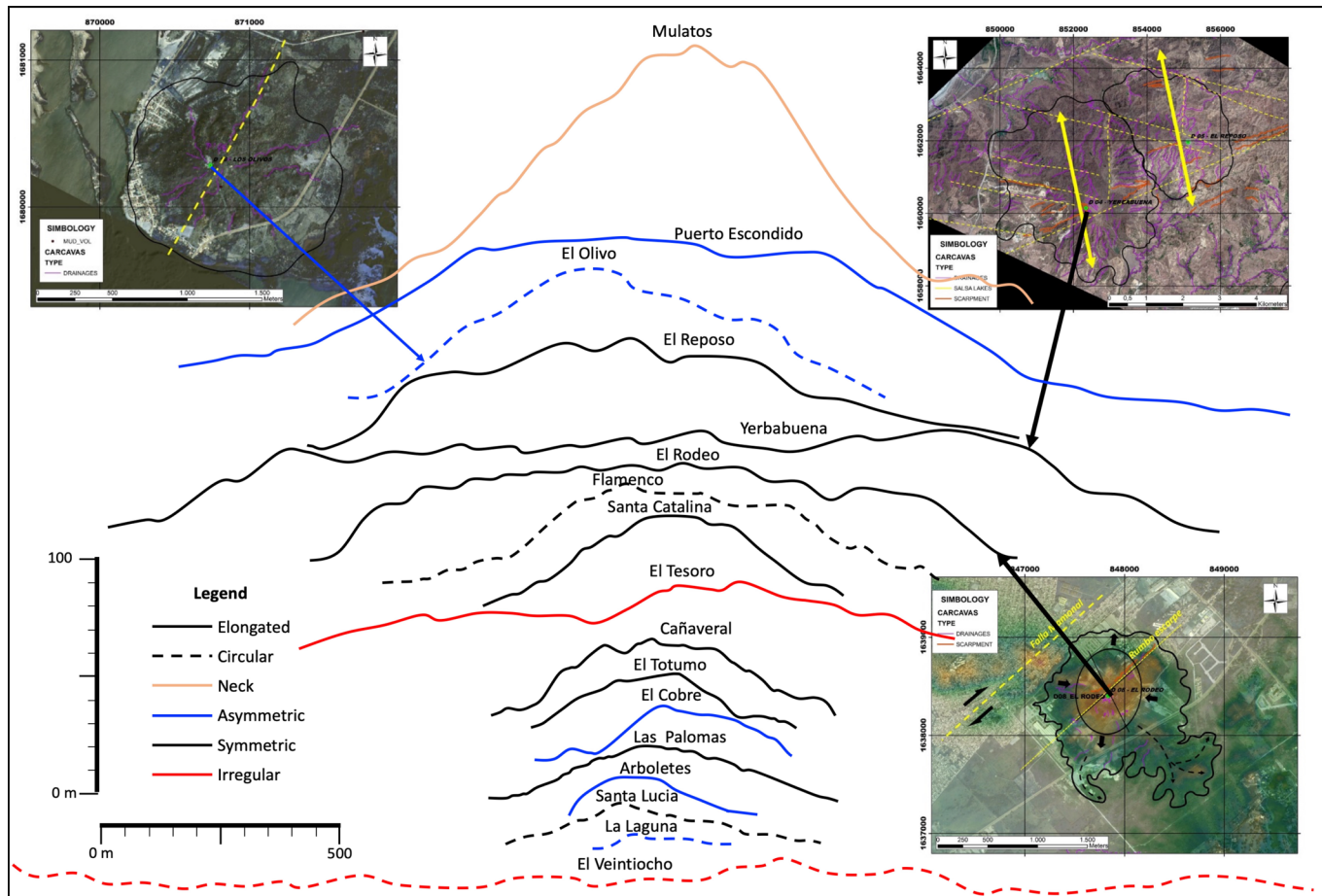
Figure 2. Average topographic profiles of the volcanoes studied in the Colombian Caribbean (extracted from Digital Elevation Models with 12 m of resolution), with their degree of ellipticity and morphology (according to the geomorphological descriptions summarized in table 2). The images show examples of some mud volcanoes with an elongate shape (right hand images), and asymmetrical circular shapes (upper left images).
