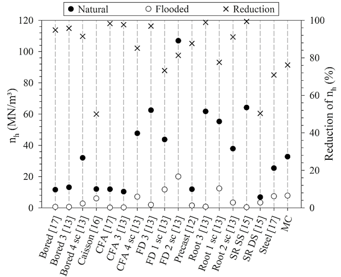
Figure 8. Comparison between n_h values from the new post-grouted micropile and from others pile types in the same subsoil profile. Source: The authors.
