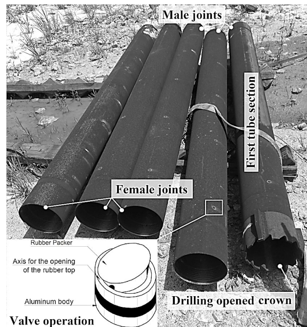
Figure 2. Lost/Structural/Drilling casing and valve in detail. Source: The authors.
