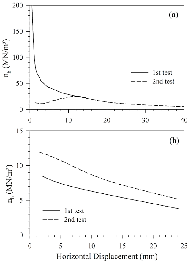
Figure 7. Graphs of n_h vs. horizontal displacement for (a) natural soil moisture content and (b) flooded conditions. Source: The authors.
