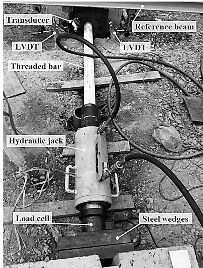
Figure 5. In-situ configuration between tested and reaction micropiles. Source: The authors.
