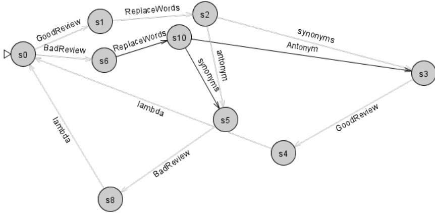
Figure 4. FVS-based Automaton
