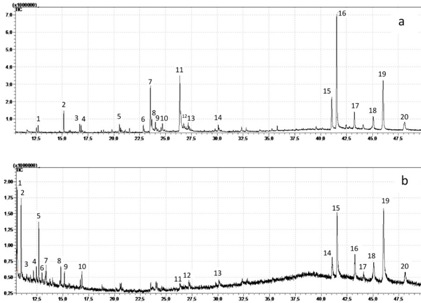
Figure 5: Chromatogram of organic compounds obtain from gadung tubers in (a) n-hexane extract (b) petroleum ether extract.
