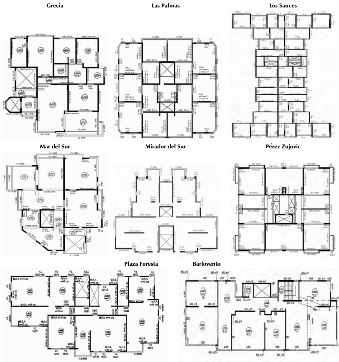
Figure 2. Typical plan view of buildings. Source: Authors
