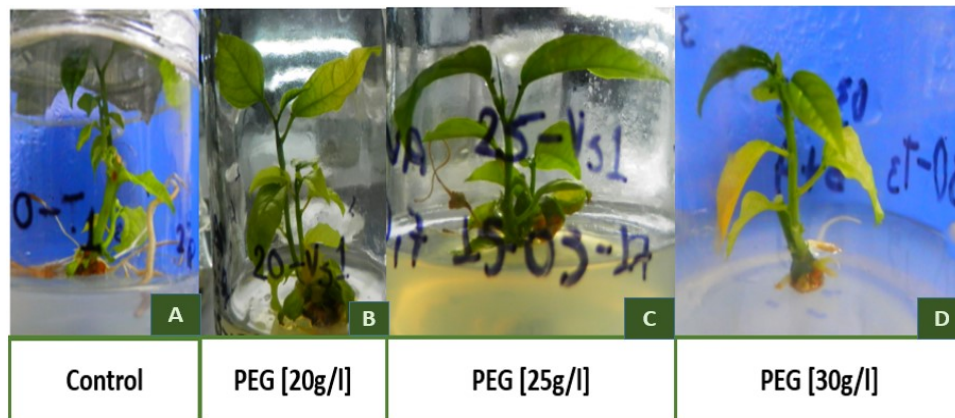
Figure 2. Comparison of leaves produced under water stress in passion fruit SV, notice the growth of leaves in PEG 20 y 25 g·L -1 treatment. A. Control treatment, B, C and D, Organogenic médium with PEG 6000 in concentrations of (0, 20, 25 and 30 g/l).
