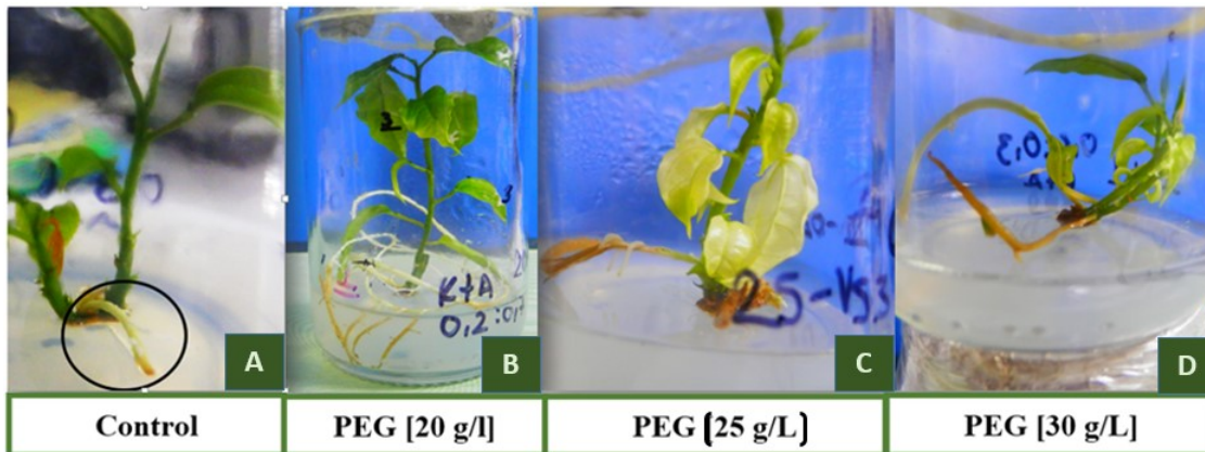
Figure 1. Longitudinal growth comparison of passion fruit SV roots in four concentration of root PEG and organogenics mediums, notice root growth and thickness concerning the control. A. Control treatment, B, C and D, Organogenic médium with PEG 6000 in concentrations of (0, 20, 25 and 30 g/l).
