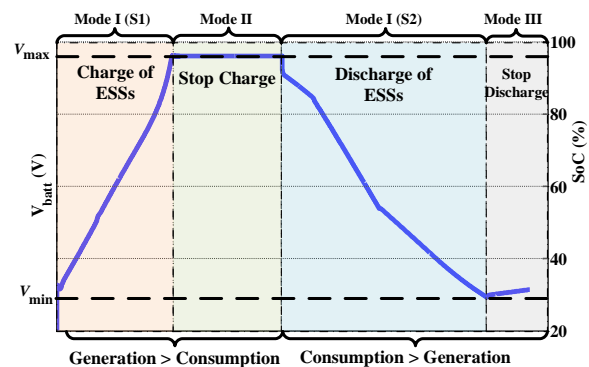
Figure 2. Desired operation Profile for the battery in the islanded microgrid.
