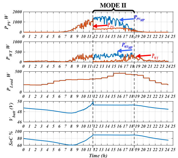
Figure 5. Operation of the microgrid for time period of 24h. Source: Authors
