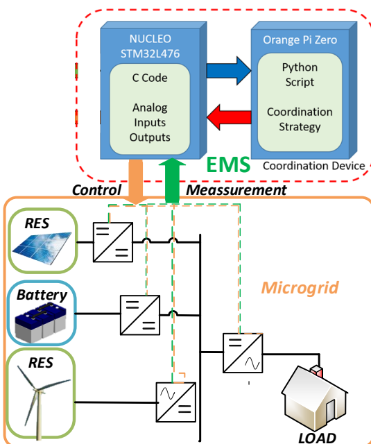
Figure 3. Structure of the EMS electronic device integrate to the microgrid.
