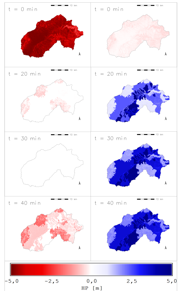
Figure 8. Maps of the spatial and temporal distribution of the pressure head: Left) on the surface, Right) at the depth of the soil layer. Source: Author
