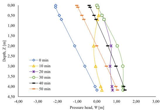
Figure 7. Response of the pressure head in a single cell. Source: Author
