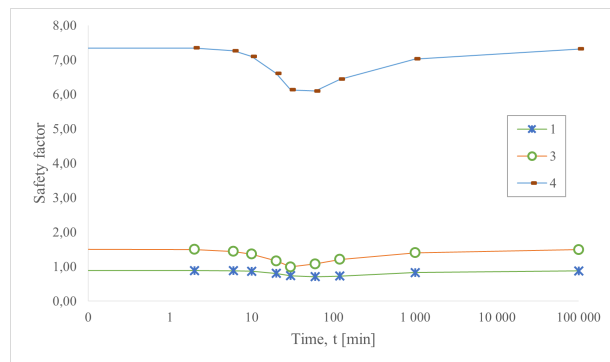
Figure 17. Recovery of the safety factor as a function of time.
