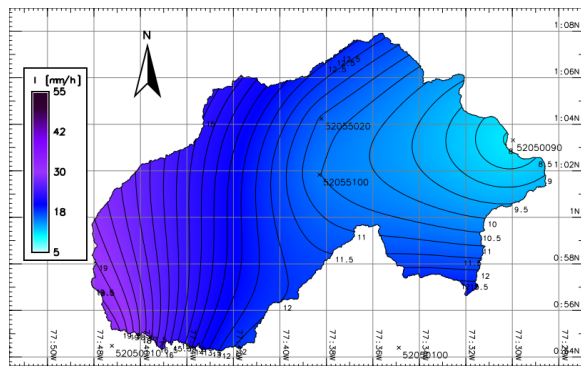
Figure 6. Rain intensity map. Source: Author
