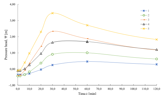
Figure 9. Temporal changes of head of pressure on individual slopes for a rain of 30 minutes in 5 individual slopes. Source: Author
