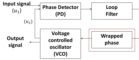
Figure 2. Second-level PLL with a wrapping phase algorithm. Source: Authors
