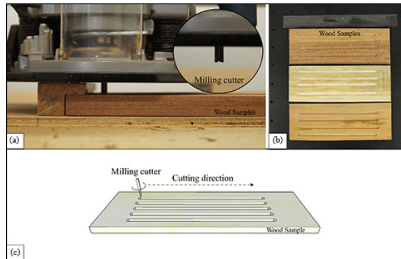
Figure 1: Mechanical processing done with a router. (a) End mill cutter on wood samples. (b) Wood samples of the three species after milling. (c) Outline of the specimen after consecutive cuts of the milling machine.
