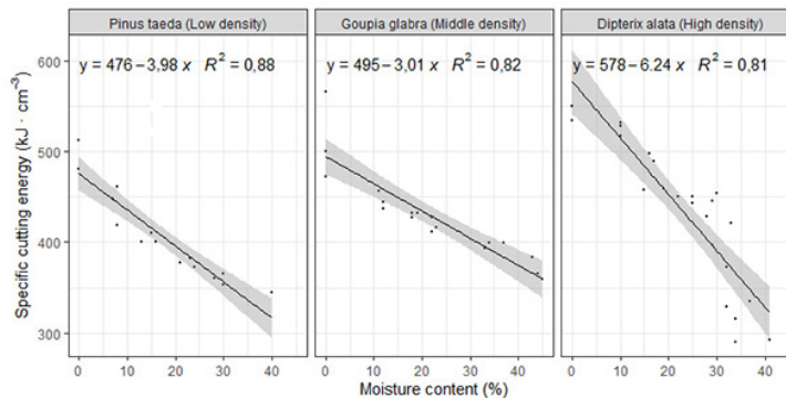
Figure 3: Behavior of specific cutting energy with moisture content variation for species of three densities.
