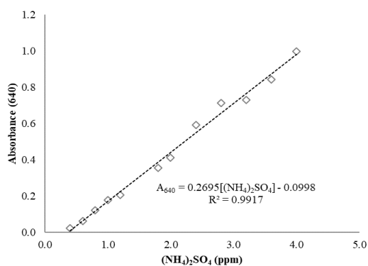
Figure S2. Calibration curve for ammonium quantification. Source: The Authors.
