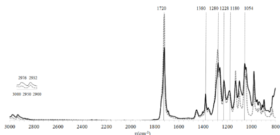
Figure S4. FTIR spectra for PHB commercial (.....) and PHB produced by B. megaterium LVN01 from waste glycerol (—). Source: The Authors.
