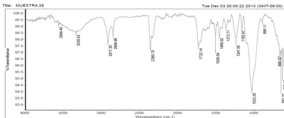
Figure 7. FTIR analysis of the citric acid modified palm bagasse.
