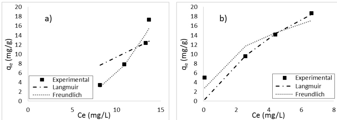
Figure 6. Adsorption isotherms adjustment for the adsorption of Hg(II) onto (a) unmodified palm bagasse peels, and (b) palm bagasse modified with citric acid.
