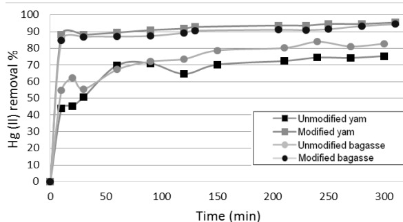
Figure 1. Adsorption kinetics of Hg(II) at pH 6,0 using yam peel and palm bagasse biomass modified with citric acid.
