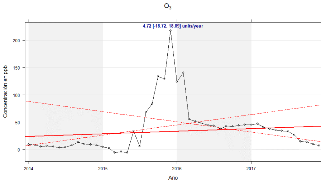
FIG. 6 Trend of daily concentrations for O_3 in ITVH. Period 2014-2017.
