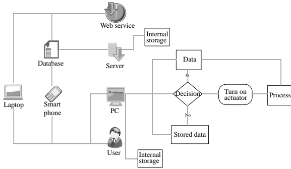
Fig. 2. Dissolved oxygen control hardware and software architecture.
