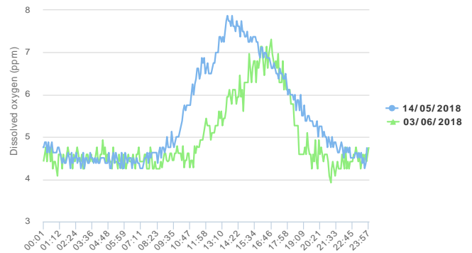
Fig. 11. Dissolved oxygen control with 4.4ppm set point
