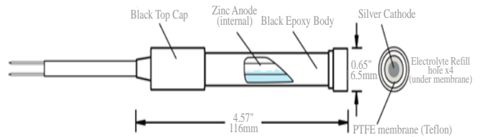
Fig. 3. Dissolved oxygen sensor Atlas Scientific [12].
