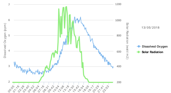
Fig. 6. Dissolved oxygen vs Solar Irradiance.
