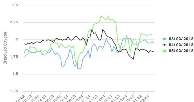
Fig. 1. Dissolved oxygen record in a geomembrane tank without control for 3 days.
