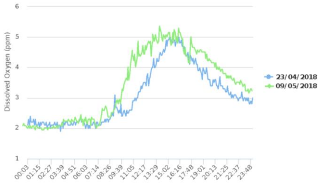
Fig. 7. Dissolved oxygen control with 2.1ppm set point
