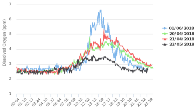
Fig. 8. Dissolved oxygen control with 2.5ppm set point
