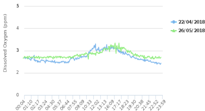
Fig. 9. Dissolved oxygen control with 2.8ppm set point
