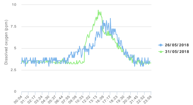
Fig. 10. Dissolved oxygen control with 3.5ppm set point
