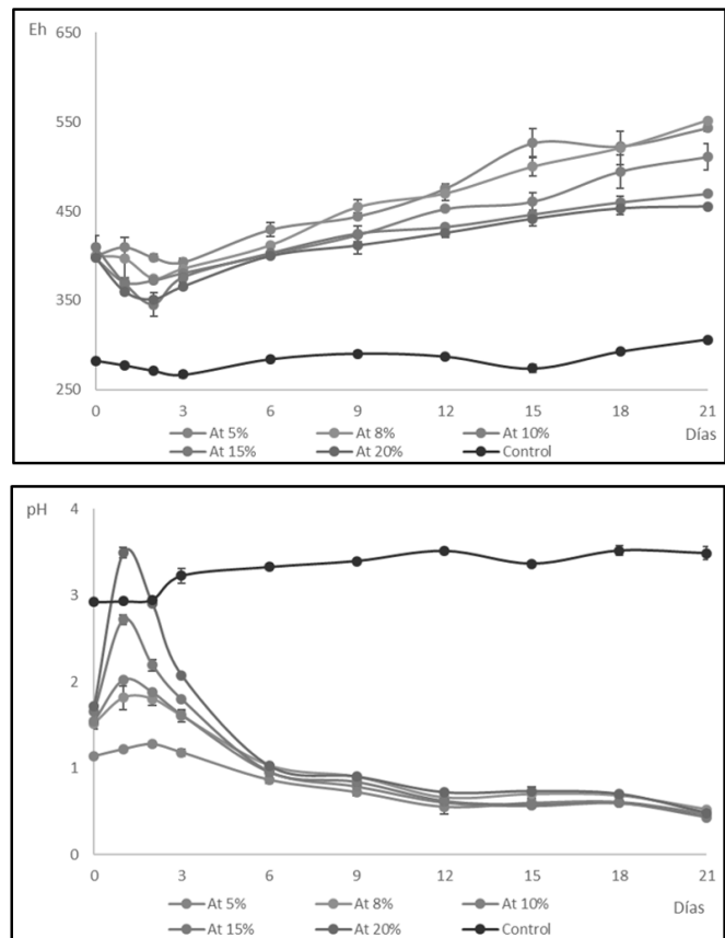
Figure 6. a) Eh curve for the bioleaching process by A. thiooxidans . b) pH curve for the bioleaching process by A. thiooxidans .
