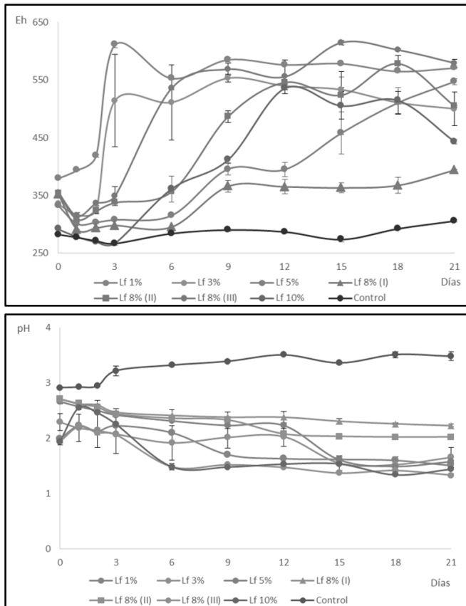
Figure 5. a) Eh curve for the bioleaching process by L. ferrooxidans . b) pH curve for the bioleaching process by L. ferrooxidans .
