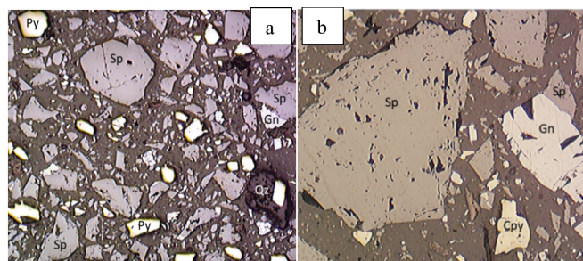
Figure 1. MOLPP images. a) 40X magnification. High concentration of sphalerite grains (Sp, blue-grey); inter-growth of sphalerite grain next to galena grain (Gn, upper and lower left). Pyrite grains (Py, brass yellow) with high reflectance. b) 100X magnification. Sphalerite grain with some porosity. Galena grain with triangular holes caused by polishing and cubic cleavage, with simple inter-growth next to sphalerite grain. Chalcopyrite grain.
