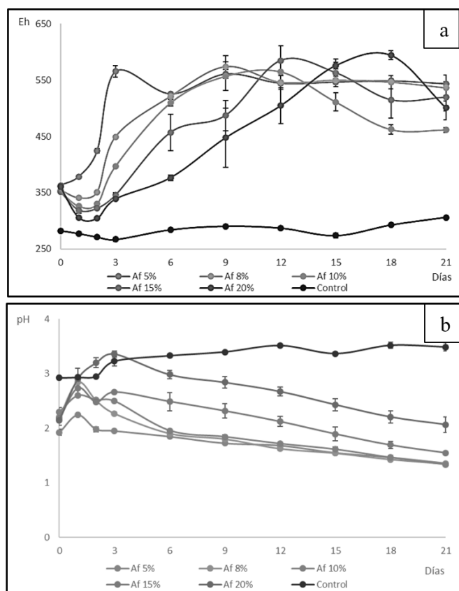
Figure 4. a) Eh curve for the A. ferrooxidans bioleaching process. b) pH curve for the A. ferrooxidans bioleaching process.
