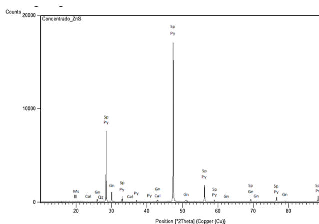
Figure 2. X-ray diffractogram of the concentrated sphalerite sample. (Sp: sphalerite, Py: pyrite, Cpy: chalcopyrite, Gn: galena, Qz: quartz, Ill: Illite, Ms: Muscovite, Calcite).
