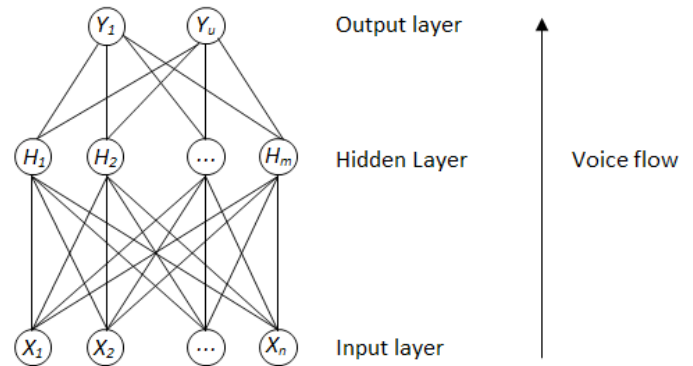
Fig. 5. Example of typical Artificial Neural Network.
