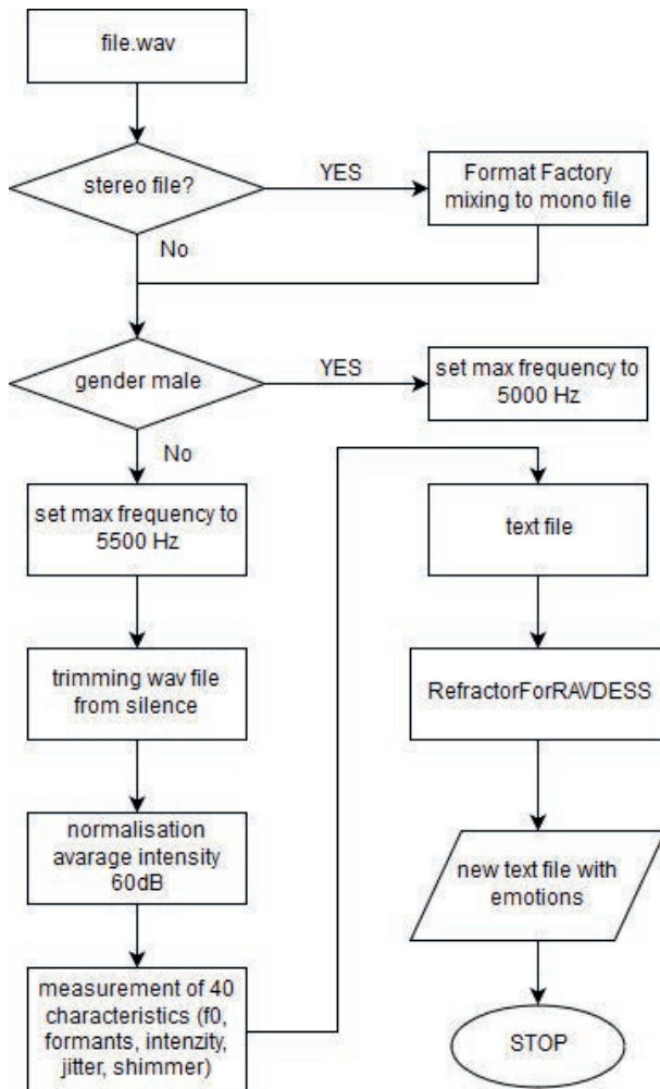
Fig. 2. The flow chart of process for extract relevant features from audio waveforms.
