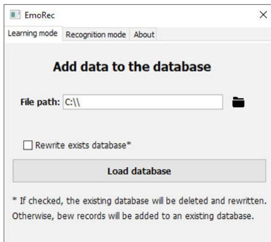
Fig.4. EmoRec – learning mode.
