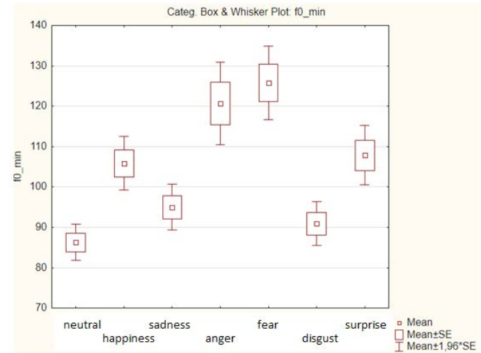
Fig. 3. Example - condition of equality of variances of characteristics f0_min is not fulfilled.
