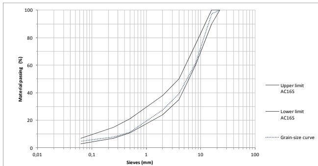
Figure 2. Particle size of the combined aggregate Source: The authors
