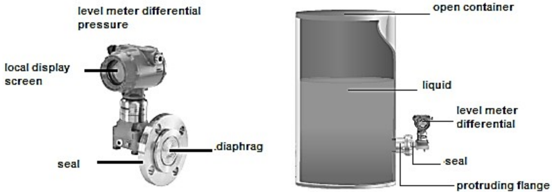
Figure 3. Level Meter differential pressure in an open container. Source: [25].
