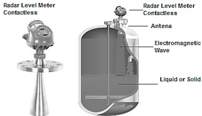
Figure 6. Radar level meter without contact. Source: [25].
