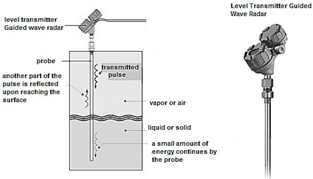
Figure 5. Level Meter guided wave radar. Source: [33], [34].
