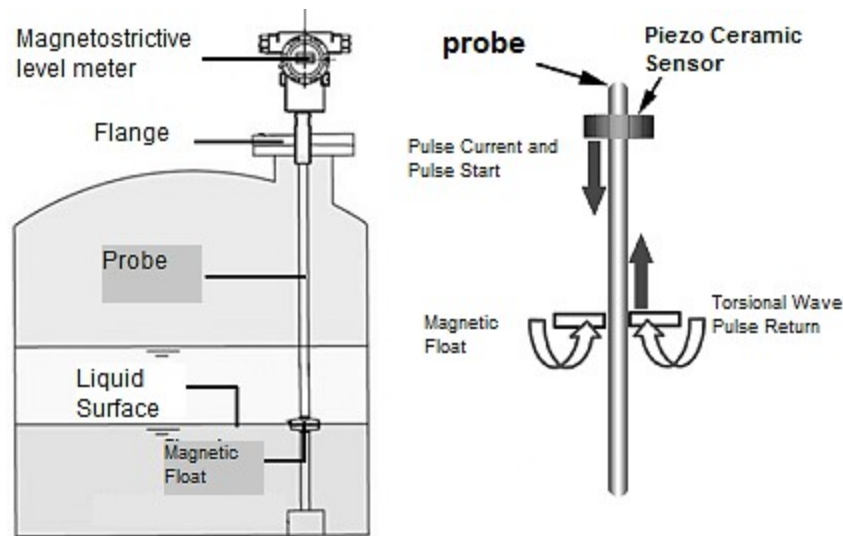
Figure 11. Magnetostrictive level meter. Source: [54], [28].
