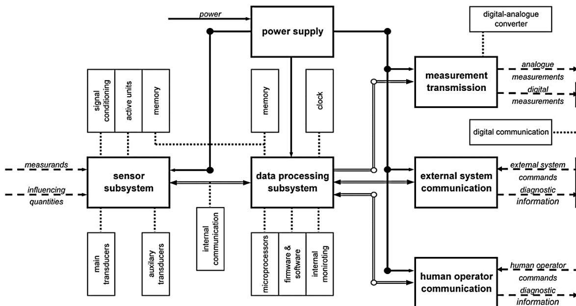
Figure 1. Schematic of operation of a smart transmitter. Source: [19], [20].
