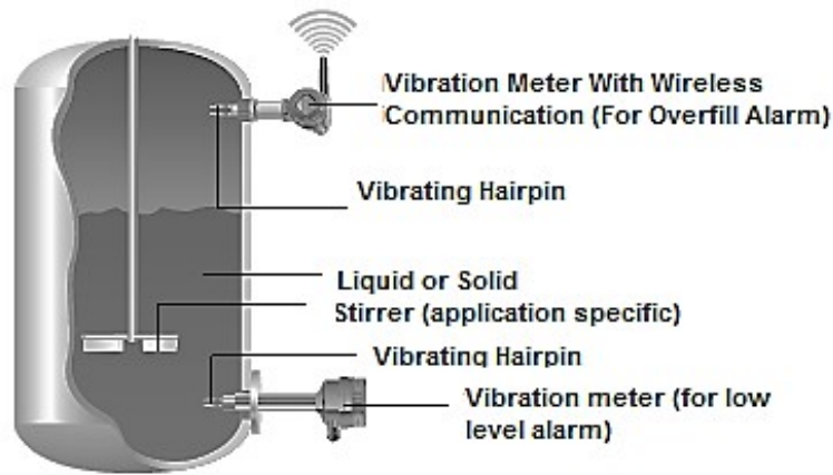
Figure 13. Vibrating level switch for alarm application. For low-level and high-level alarm [25].
