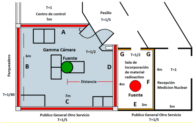
Figure 1 Structural plan, gamma chamber ward (
