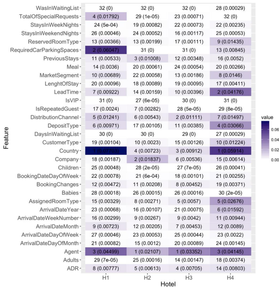
Figure 5: Mutual information feature selection filter results (order and value)
