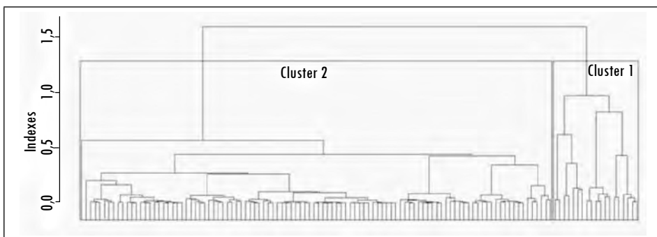
Figure 3. Dendrogram
