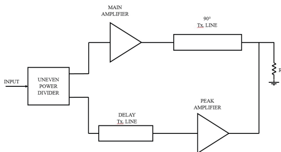
Fig. 4. General scheme of a DPA. Source: Authors.
