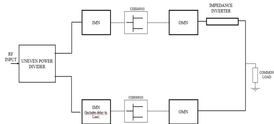
Fig. 11. Scheme of the designed DPA. Source: Authors.
