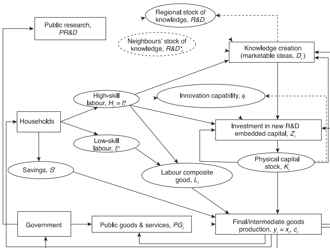
Figure 1. Schematic representation of the economy in RHOMOLO
