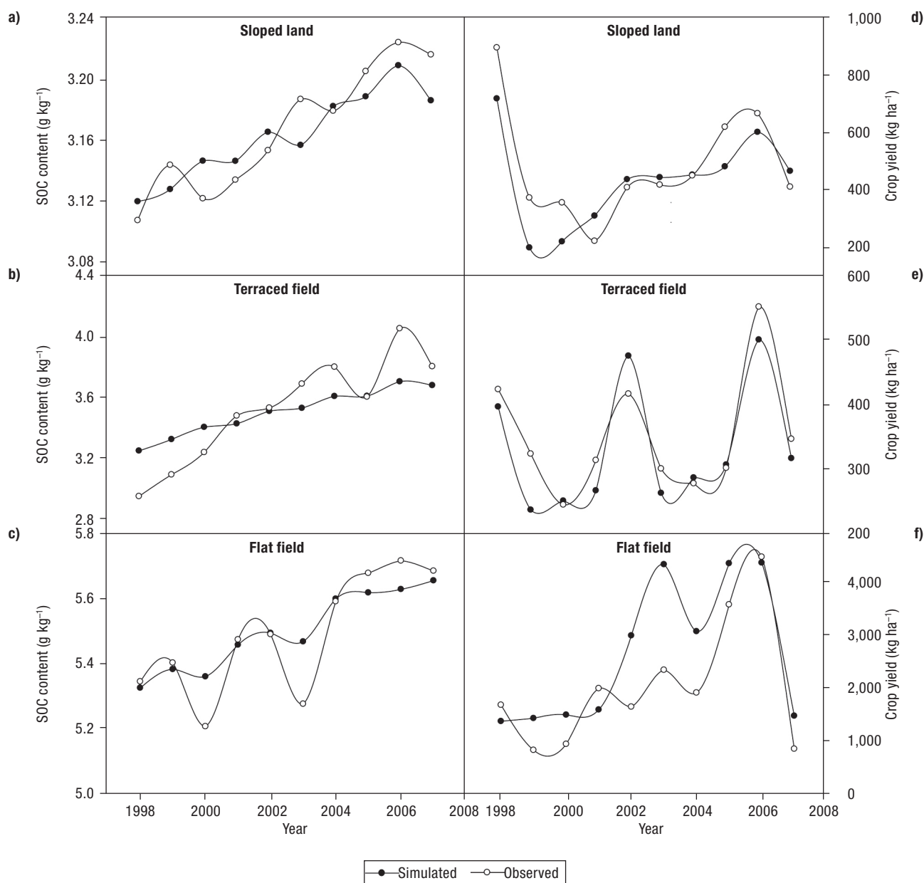
Figure 2. Changes of observed (0-30 cm) and DNDC model simulated soil organic carbon (left) and crop yield (right) over time, from 1998 to 2007 under single manure fertilization (7,500 kg ha -1 farmyard manure containing 15.9% organic matter and 1.3% N) in sloped land (a, d), terraced field (b, e) and flat field (c, f).
