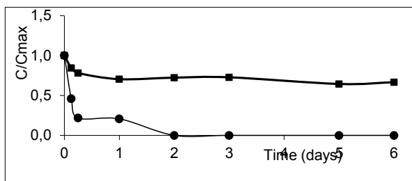
Figure 3. Variation in C/C_{max} of the different compounds detected in the liquid culture obtained from the microbial consortia of agricultural soils exposed to MP. Symbols: (■) MP; (●) PN.
