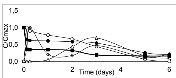
Figure 2. Variation in C/C_{max} of the different compounds detected in the liquid culture obtained from the microbial consortia solid organic waste. Symbols: (■) MP, (●) PN, (Δ) UDP 3 , (○) UDP 4 , (◇) UDP 5 .
