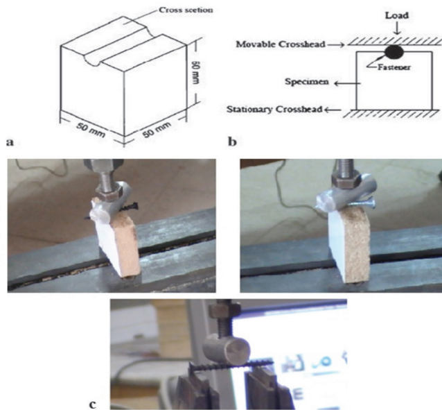
Figure 4. a. Dimensions of dowel bearing strength test. b. A schematic drawing of dowel bearing strength test setup. c. Bending yield strength of wood screw test setup
