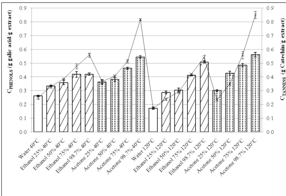
Figure 2. Effect of temperature and organic solvent concentration on the total phenol content (Acetone: ■■■ Ethanol: // and Water: □) and tannin's concentration (✱) of pine bark extracts.
