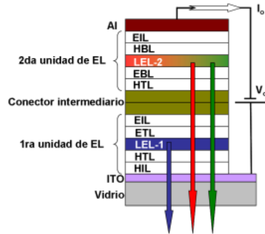
Figura 9. Estructura de un SOLED [42]. EL: emission layer; EIL: electron injector layer; HBL: hole blocking layer; LEL: light emission layer; EBL: electron blocking layer; ETL: electron transport layer; HTL: hole transport layer; HIL: hole injector layer.
