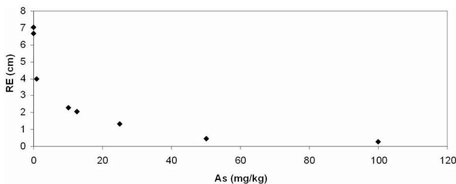
Figure 2. Root elongation (RE) in relation to the As concentration of the spiked solutions.
