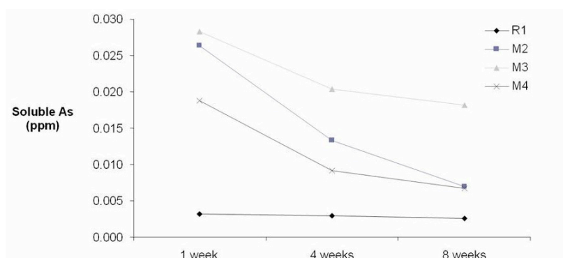
Figure 1. Soluble As concentrations in the different soils in the three incubation periods.
