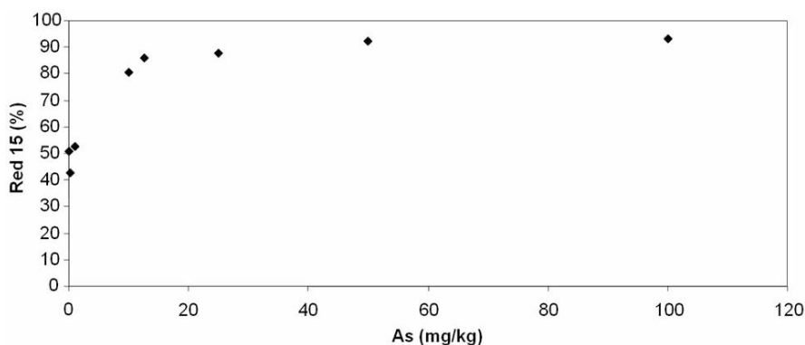
Figure 3. Percentage in reduction of luminescence (Red 15) in Microtox test in relation to the As concentration of the spiked solutions.
