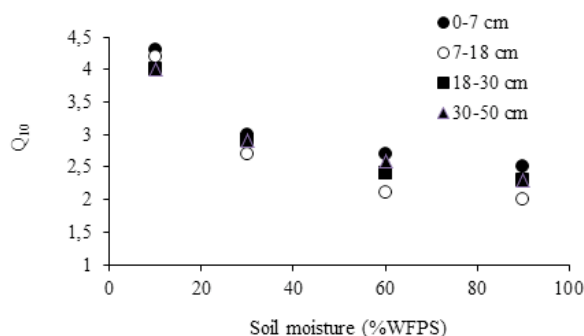
Figura 5. The temperature sensitivity ( Q_{10} ) of aerobic CO 2 production connected with soil moisture in soil samples collected at depths of 0-7, 7-18, 18-30 and 30-50 cm.
