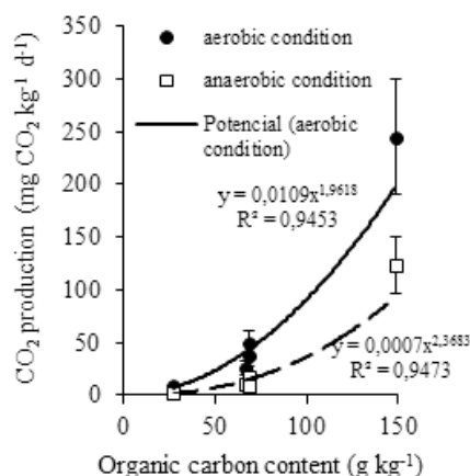
Figure 2. Relationship between CO 2 production and soil organic carbon content under aerobic and anaerobic conditions at 20 °C of temperature. Every value of CO 2 production is the average at the soil moisture range of 10-90% WFPS. Error bars indicate the standard deviation ( n = 24 ).
