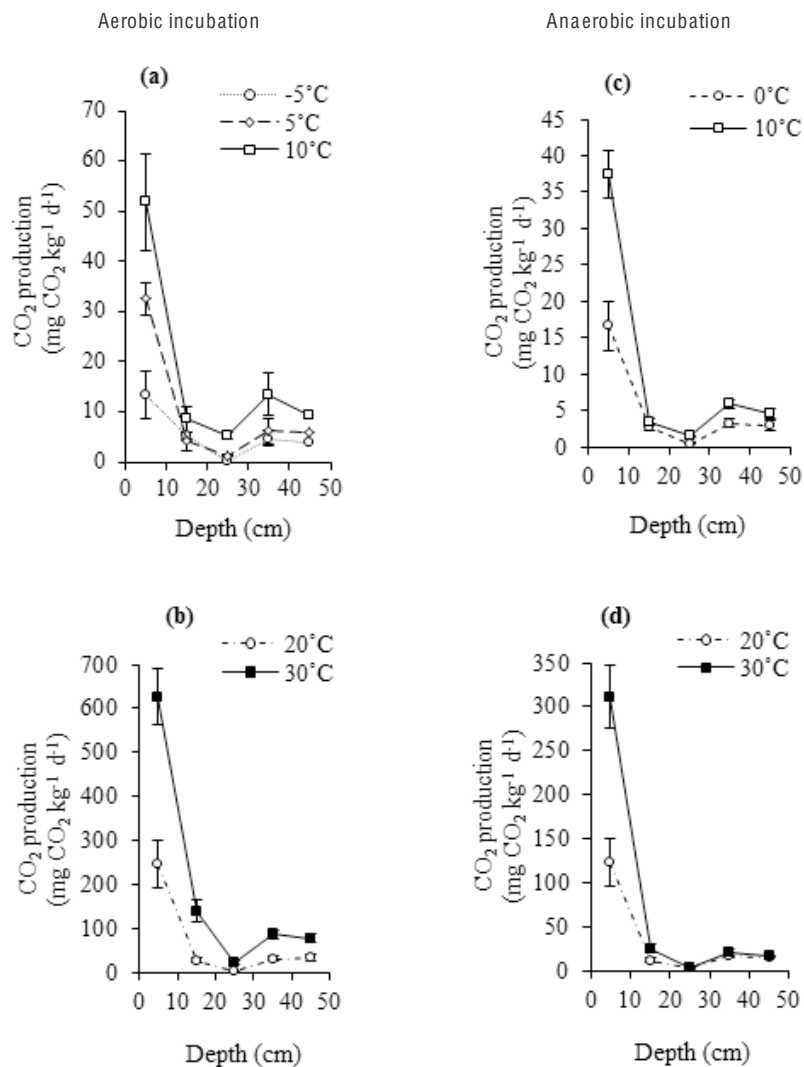
Figure 1. The CO 2 production rate connected with soil depth under aerobic (a, b) and anaerobic (c, d) conditions at different incubation temperatures. Every value of CO 2 production is the average at the soil moisture range of 10-90% of water-filled pore space (WFPS). Error bars indicate the standard deviation (n = 24).
