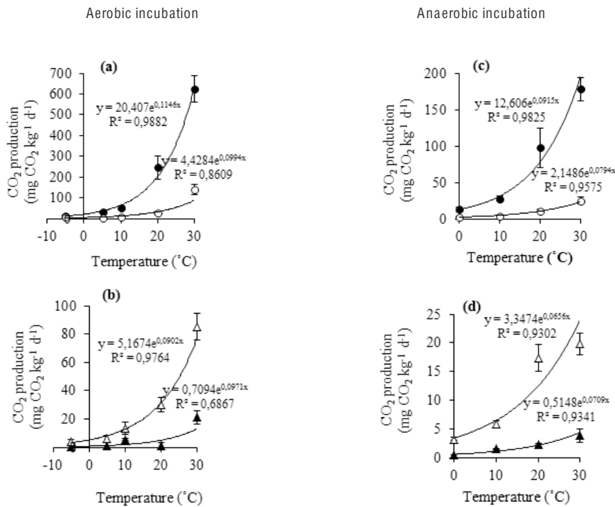
Figure 4. Relationship between CO 2 production and soil temperature. Plots show CO 2 production in the soil samples being collected at depths of 0-7 cm (filled circles), 7-18 cm (open circles), 18-30 cm (filled triangles) and 30-50 cm (open triangles), incubated under aerobic (a, b) and anaerobic (c, d) conditions. Every value of CO 2 production is the average at the soil moisture range of 10-90% WFPS. Error bars indicate the standard deviation (n = 24).
