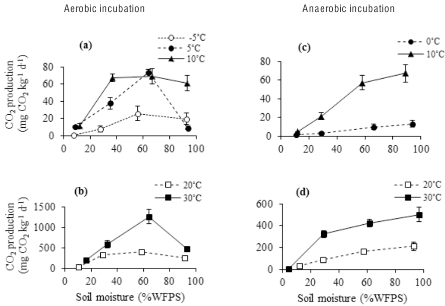
Figure 3. Relationship between CO 2 production and soil water content (water-filled pore space, WFPS) for the soil samples collected at a depth of 0-7 cm and incubated at different temperatures under aerobic (a, b) and anaerobic (c, d) conditions. Error bars indicate the standard deviation (n = 6).
