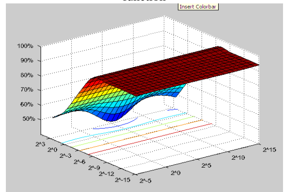
Figure 6: Surface plot for the Nu-SVM and sigmoid kernel function
