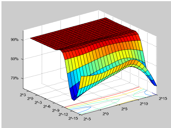
Figure 4: Surface plot for the Nu-SVM and polynomial kernel function
