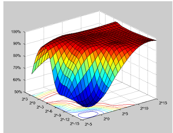
Figure 2: Surface plot for the C-SVM and RBF kernel functions
