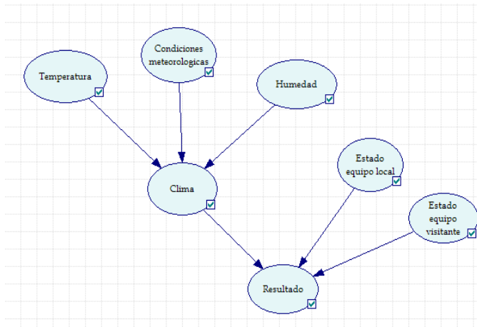
Fig. 4. Bayesian Network
