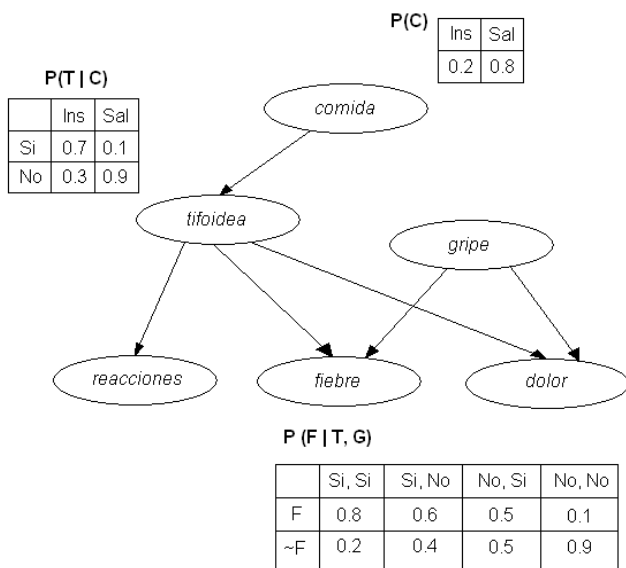
Fig. 1. Example fo bayesian network with some parameters
