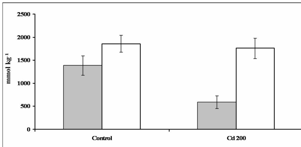
Figure 6. Content of oxalic acid and citric acid in stems of tumbleweed plants exposed for 48 h to 0 and 200 mg Cd L -1 . Data are mean of 3-4 replicates \pm S.E.
