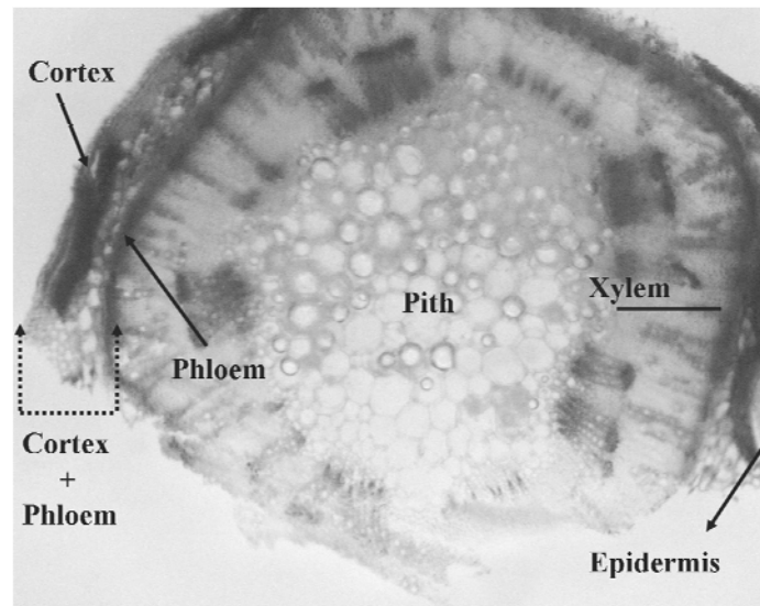
Figure 1. Cross section of native tumbleweed stem stained with Read Ponceau. Different tissues are indicated.
