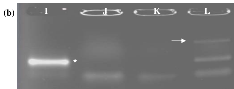
Figure 5. (a) PCR using primers of Arabidopsis thaliana and Zea mays . A, tumbleweed DNA + Arabidopsis thaliana primers; B, Zea mays DNA + MP1 ‡ ; C, tumbleweed DNA + Zea mays primers; D, corn truffle DNA + MP1 ‡ ; E, alfalfa DNA + MP1 ‡ ; F, positive control; G, molecular weight marker; H, MP1. (b) PCR using degenerated primers of the Brassica family. I, MP2 § ; J, tumbleweed DNA + PEIF; K, tumbleweed DNA + PEIB; L, tumbleweed DNA + MP2 § . ‡ Arabidopsis thaliana + Zea mays primers; § PEIF + PEIB. Arrow shows a potential amplicon; Asterisk indicates primer/dimer artifact.
