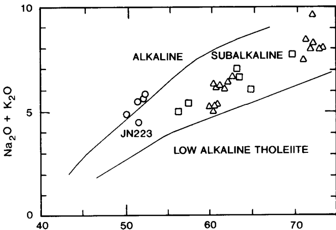
Figure 6. Alkali vs. silica. Fields given for alkaline, subalkaline, and low alkaline tholeiite after Irvine and Barager (1971) and Kuno (1968). (After Neuhaus, 1989, fig. 10). Open circle: basaltic andesite; open square: andesite; open triangle: rhyolite. Sample JN 223 is subalkaline and contains greater amounts of plagioclase than other basalts analyzed.
