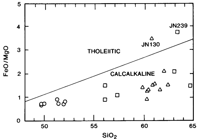
Figure 7. FeO*/MgO/SiO 2 , separation into calc-alkaline and tholeiitic fields after Miyashiro (1974). FeO* = total iron as FeO. Open circle: basalt; open square: andesite; open triangle: rhyolite. The southwestern Isla Tiburón volcanic suite has primarily a calc-alkaline trend, with the exceptions of two tholeiitic samples: JN 130 (Unit M1b) and JN 239, a dacite ash flow tuff dated at 4.16 ± 1.81 Ma (Neuhaus, 1989, fig. 3b).
