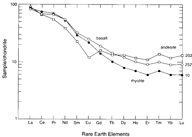
Figure 11. Spider diagram showing normalized rare earth element analyses for three rocks from southwestern Isla Tiburón, Sonora, Mexico. Normalization according to Boynton and Warrick (1984). Black circle: rhyolite; open circle: basalt; open square: andesite.
