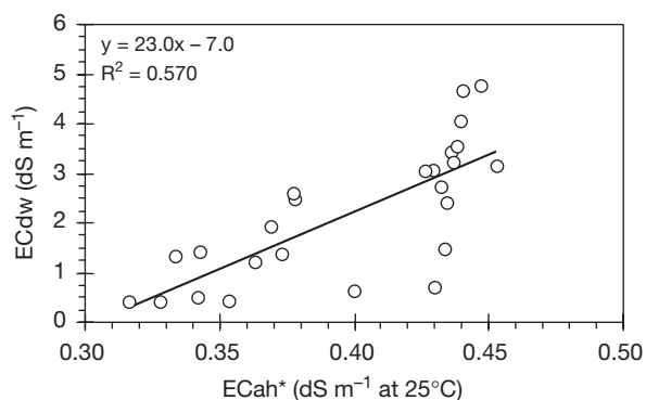
Figure 4. Relationship between drainage water salinity (ECdw) and surface-weighted apparent soil electrical conductivity (ECah*) for the 25 watersheds delimited in the Barranco de Lerma study area.
