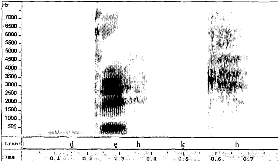
(5) Spectrogram of MP's production of the word dück 'deck'.
