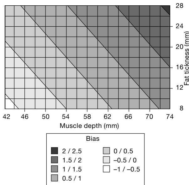
Figure 2. Contour plot of the bias obtained after a simulation study with the present equation. Bias is presented as a function of fat thickness and muscle depth.
