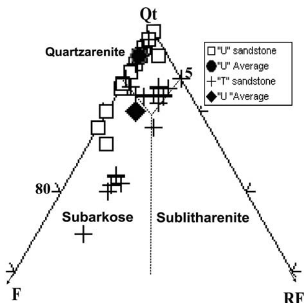
FIGURE 3 | Detrital composition of representative sandstones from the Napo Formation, plotted on Qt-F-RF (Dott, 1964 and modified by Pettijohn, 1972). Abbreviations: Qt: Quartz; F: Feldspar; RF: Rock fragments.
