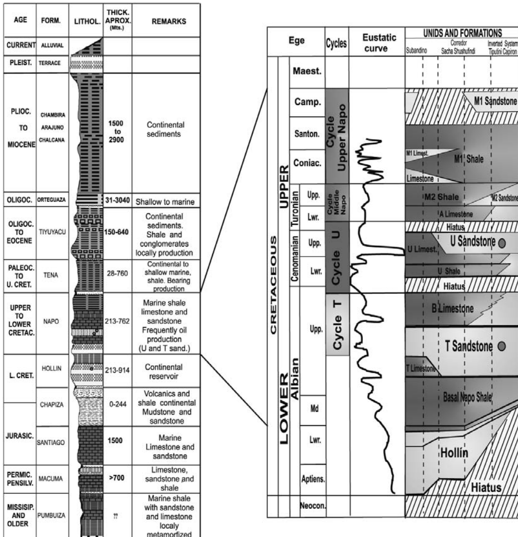
FIGURE 2 | General stratigraphical column of the Oriente Basin with lithostratigraphic nomenclature (modified from Almeida, 1986). Detailed chart showing the reservoirs “U” and “T” sandstones from the Napo Formation [after Christophoul and Rivadeneira (1986)] modified from Jaillard, 1997).
