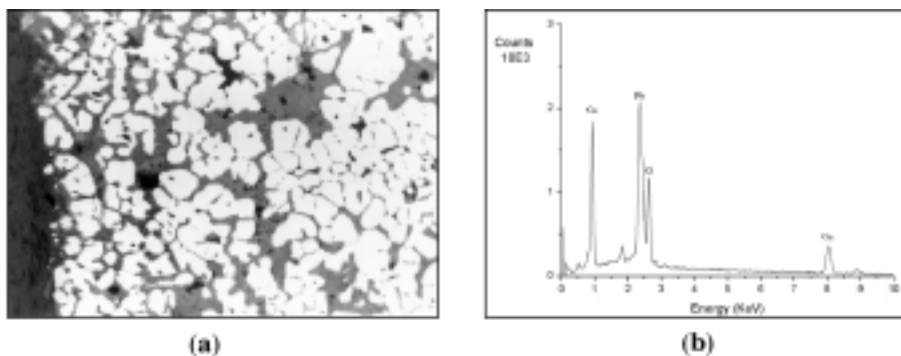
Figure 3. Macrography showing the preferential attack to segregated lead (a). EDS analysis of the preferential attack corrosion products (b).
