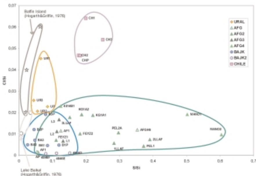
Figure. 2. Discrimination of the investigated lapis lazuli samples according to their Cl/Si. vs. S/Si ratios.
