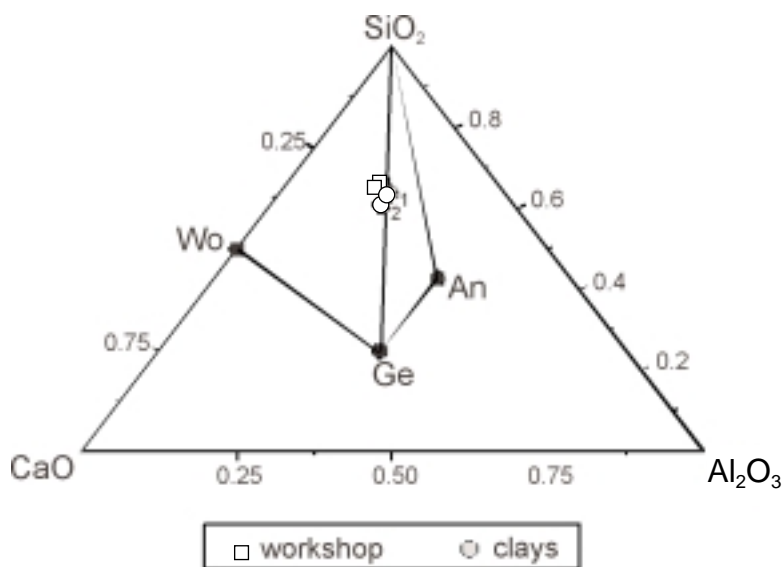
Figure 1. Chemical composition of shards and of representative clay samples reported on the ACS ( \text{Al}_2\text{O}_3 - \text{CaO} - \text{SiO}_2 ) diagram. The clay samples show different calcite amounts (25% in clay type 1 and 29% in clay type 2). In the graph the bulk composition of the shards and selected clay samples lay in the area of pertinence of typical calcareous illitic clays (after Heimann, 1989).
