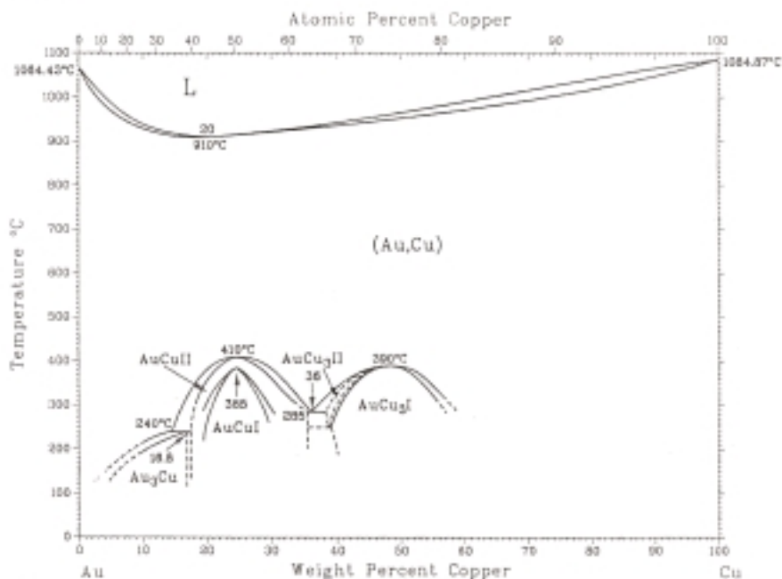
Figure 10. Au-Cu binary phase diagram showing a depressed melting point at around 10% Cu.
