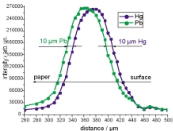
Figure 4. Depth profile showing two successive layers of cinnabar and lead white with 10 µm thickness each.
