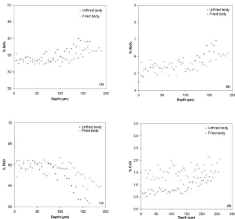
Figure. 2. Diffusion profiles of silicon (a), aluminium (b), lead (c) and calcium (d) only in the glaze area (from the glaze surface to the interface. For these samples, glazing mixture composition is: 60% PbO, 25% SiO 2 , 5% Al 2 O 3 and 10% Na 2 O and the glazes were fired with a thermal path with three firing stages.
