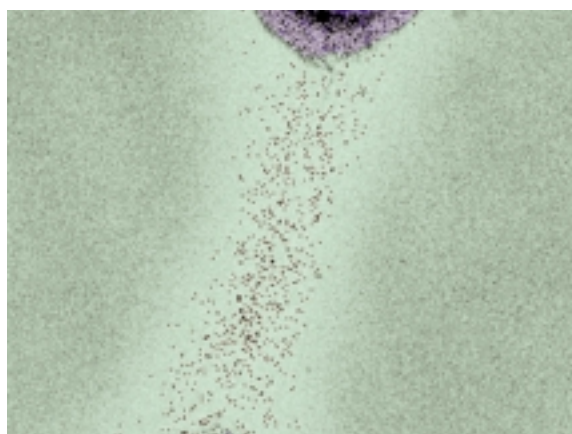
Figure 8. LISPIX compositional map showing almost 10% Cu at the granulation joint.
