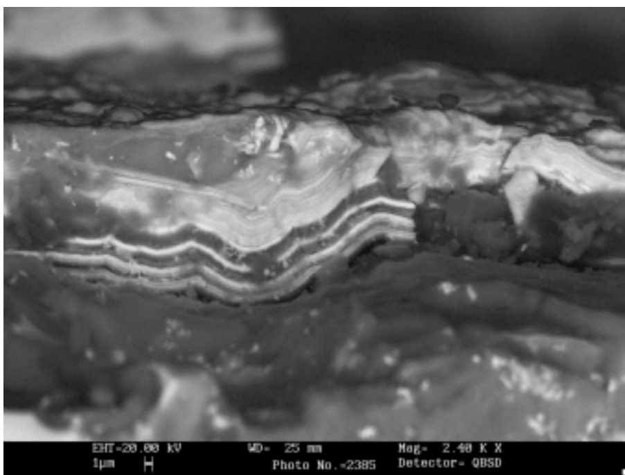
Figure 3. Glaze: study of transversal section by SEM/EDX (Backscattered electron image).
