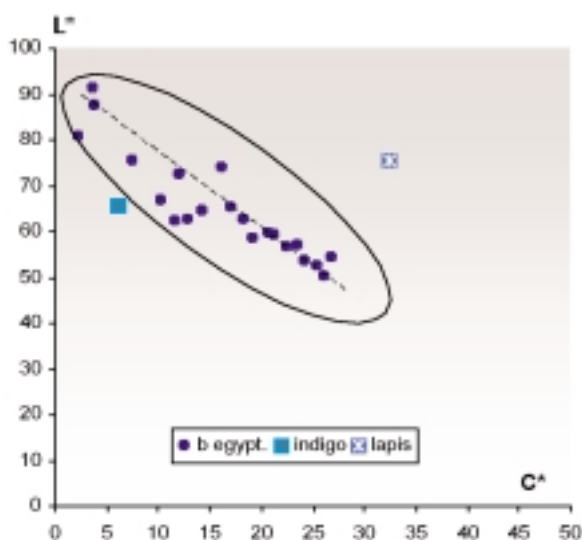
Figure 5. Colorimetric graph in C*L* coordinates of measurements on blue letters of BMO 127 (Egyptian blue) compared to lapis and indigo.
