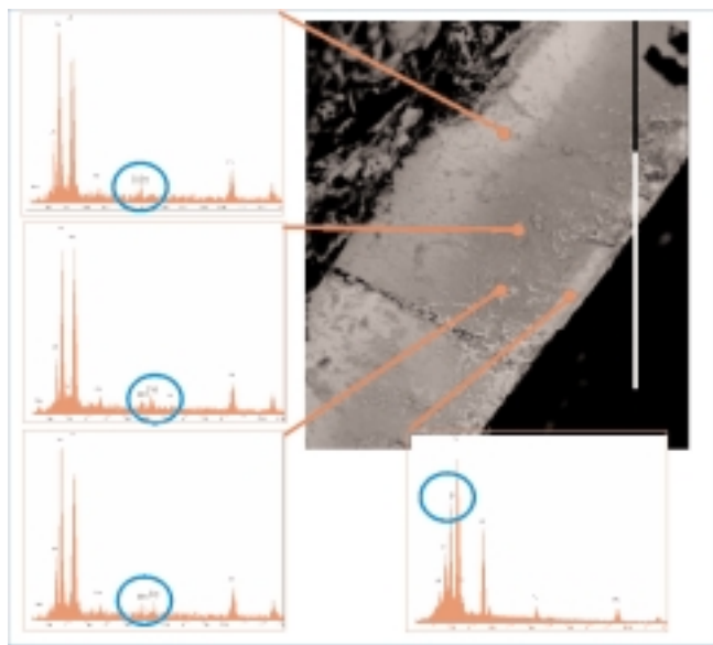
Figure 4. SEM-EDS on AMD2 specimen.
