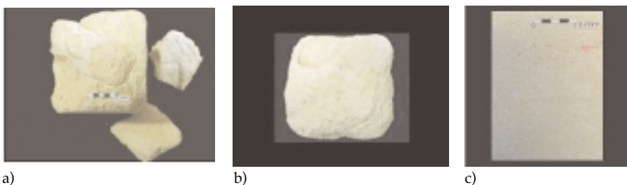
Figure 3. a) Yellowish calcarenite after 10 cycles of salt crystallisation test; b) Pale cream calcarenite at the end of salt crystallisation test (15 th cycle); c) Pale cream calcarenite at the end of resistance to ageing by SO 2 action in presence of humidity.
