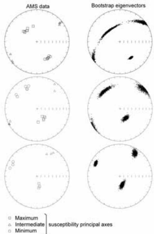
FIGURE 3 | Anisotropy of Magnetic Susceptibility data of three representative sites (see Table 1). For each site, the equal area lower hemisphere projections of the principal (squares), major (triangles) and minor (circles) eigenvectors are shown on the left. To the right are corresponding bootstrapped eigenvectors.
