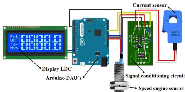
Fig. 4. Assembly diagram for power and torque meter.
