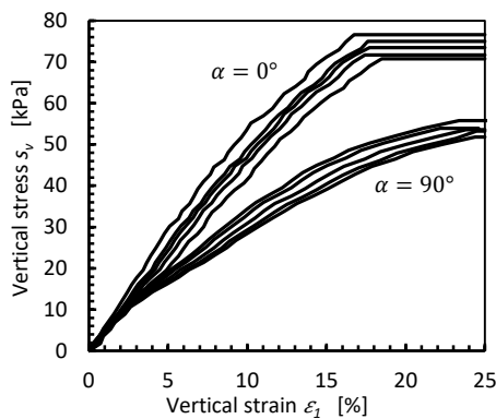
Figure 7. Unconfined compression test results of Kaolin clay. Source: The Authors.
