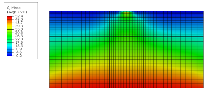
Figure 14. Contours of the deviator stress q = \sqrt{3/2} \|\sigma^*\| . Values in kPa. Source: The Authors.
