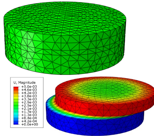
Figure 11. Finite element model for the direct shear test. Top) mesh of the model. Bottom) contours of displacements at the end of the simulation for \alpha = 0 .
