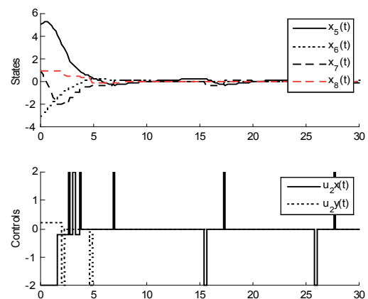
Figure 7. Status and control signal for agent 1
