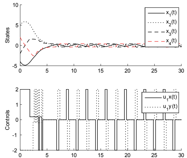
Figure 6. Status and control signal for agent 1
