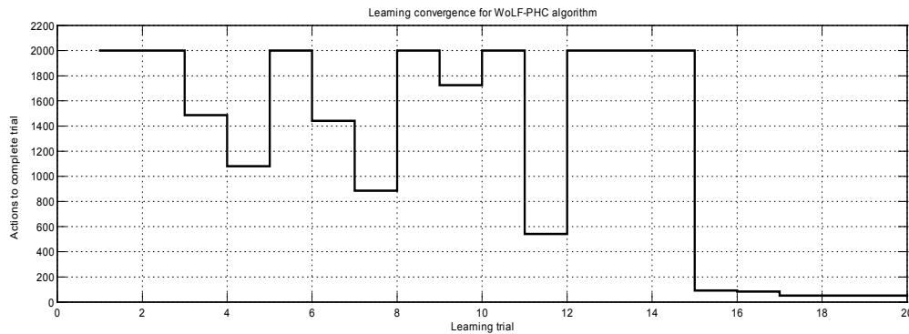
Figure 3. Convergence of the opposed algorithm
