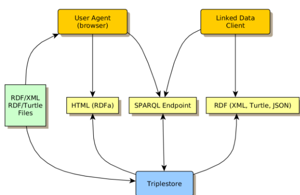
Figure 1: Functional diagram for data access of UNESKOS project. Source: PASTOR-SÁNCHEZ et al., 2013.
