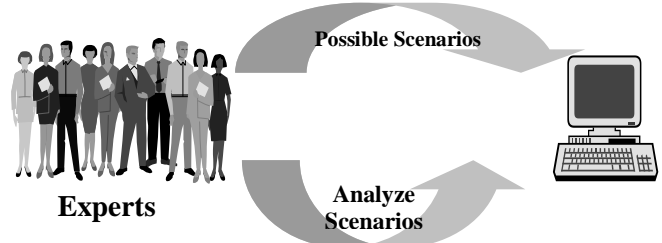
Figure 2. Knowledge extraction
