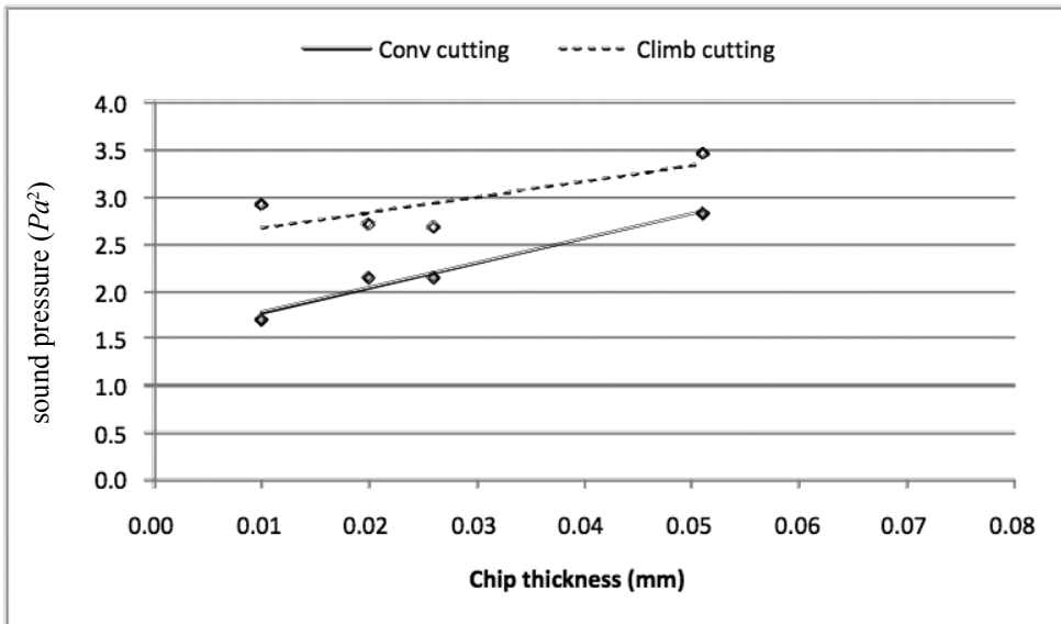
Fig 6. Sound pressure by chip thickness for conventional and climb cutting mode at 62.8 m/s of cutting speed
