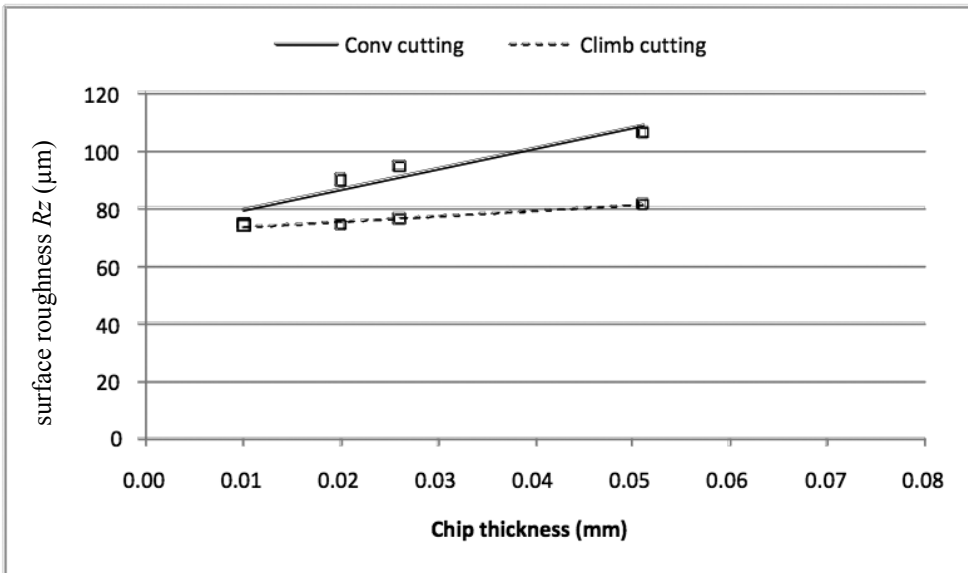
Fig 5. Surface roughness by chip thickness for conventional and climb cutting mode at 62.8 m/s of cutting speed
